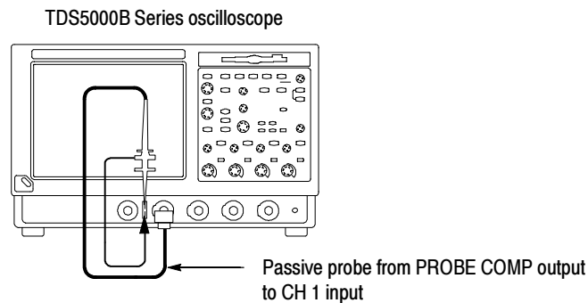
Figure 2-25: Initial test hookup
