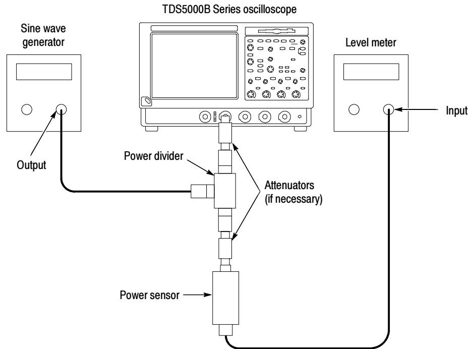
Figure 2-29: Sine wave generator leveling equipment setup (Method A)
