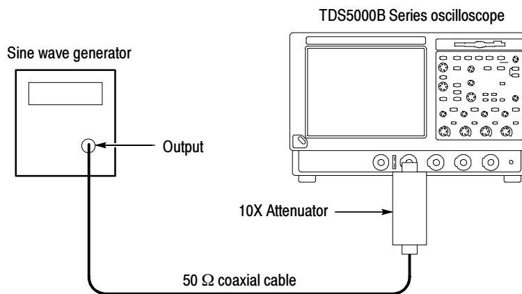
Figure 2-19: Initial test hookup
