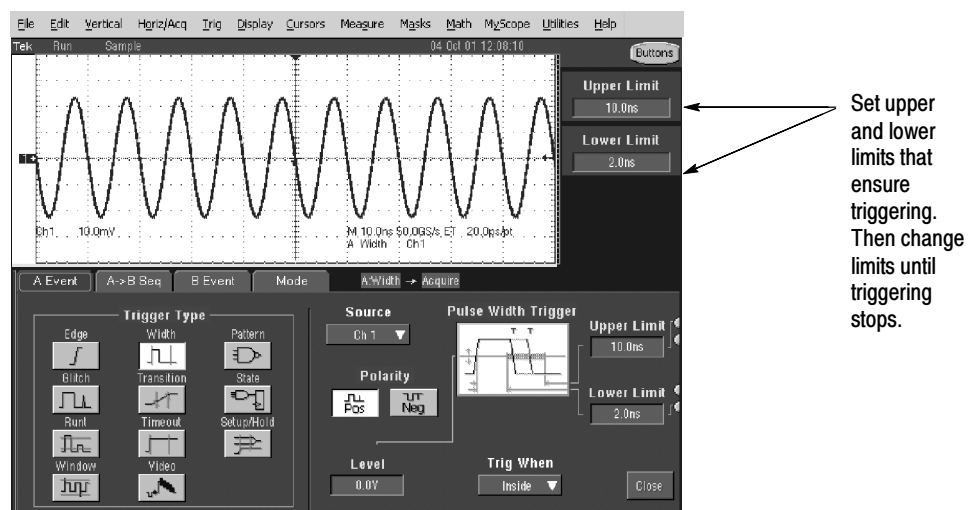
Figure 2-20: Measurement of time accuracy for pulse and glitch triggering
