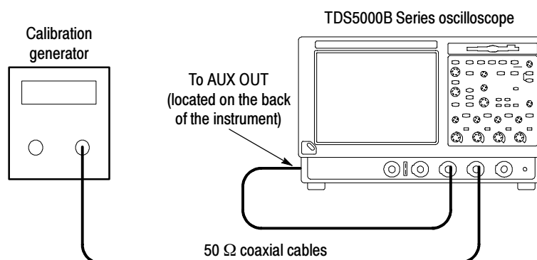
Figure 2-23: Initial test hookup
