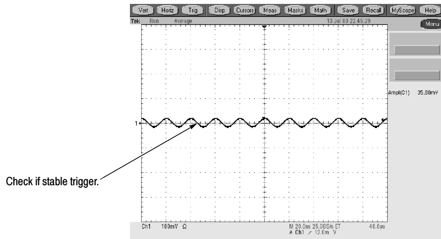
Figure 2-22: Measurement of trigger sensitivity showing 50 MHz results
