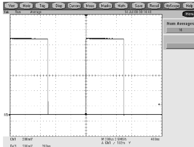
Figure 2-28: Measurement of probe compensator amplitude
