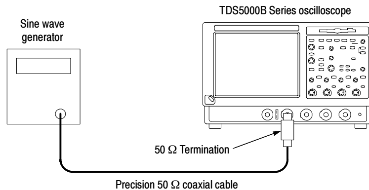
Figure 2-21: Initial test hookup
