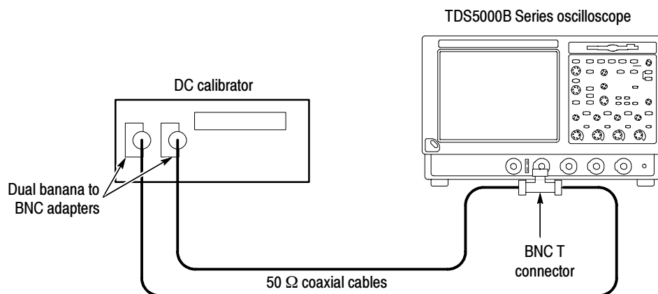
Figure 2-27: Subsequent test hookup
