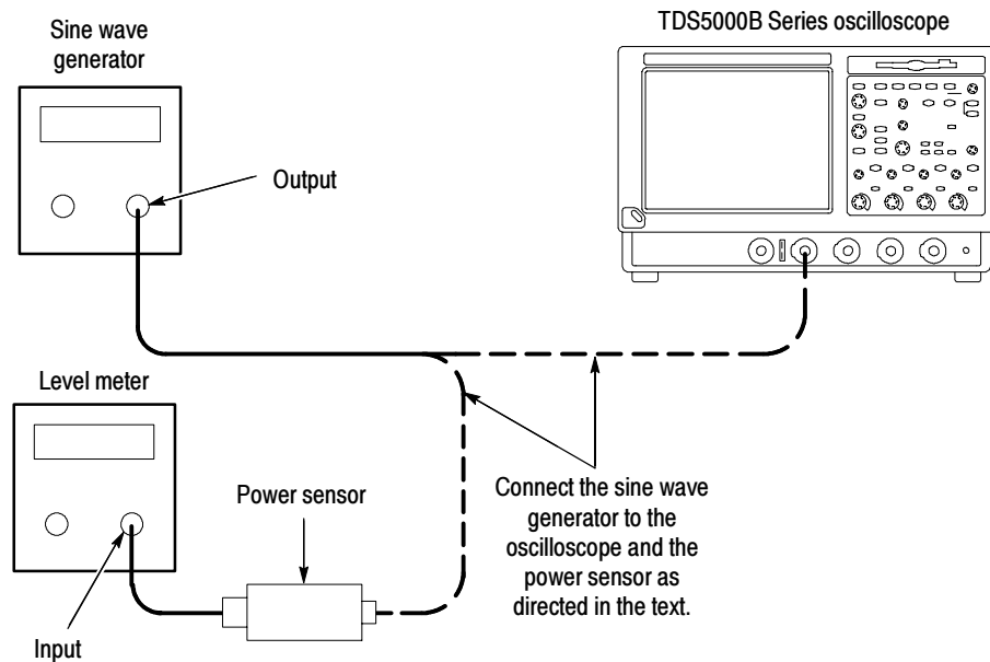
Figure 2-30: Sine wave generator leveling equipment setup (Method B)
