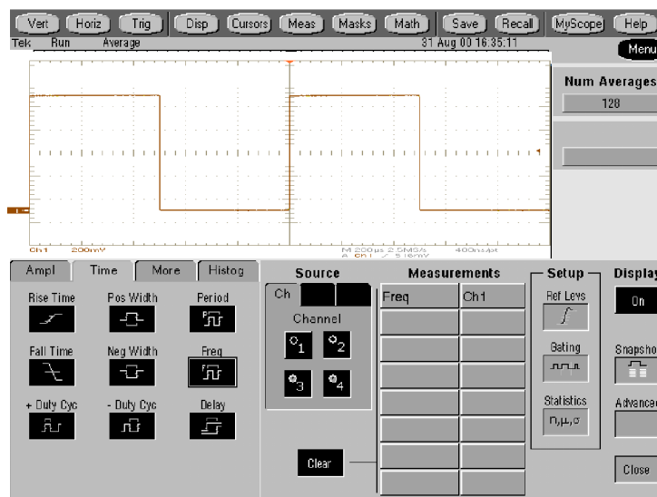
Figure 2-26: Measurement of probe compensator frequency
